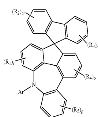
[Chemical Formula 1]
